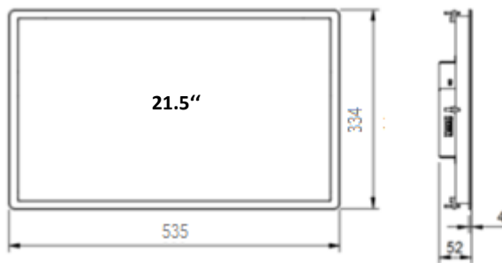
21.5" cut-out dimensions: 315mm x 516mm
