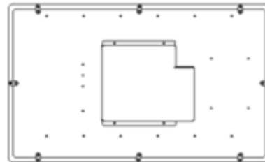
21.5" cut-out dimensions: 315mm x 516mm
